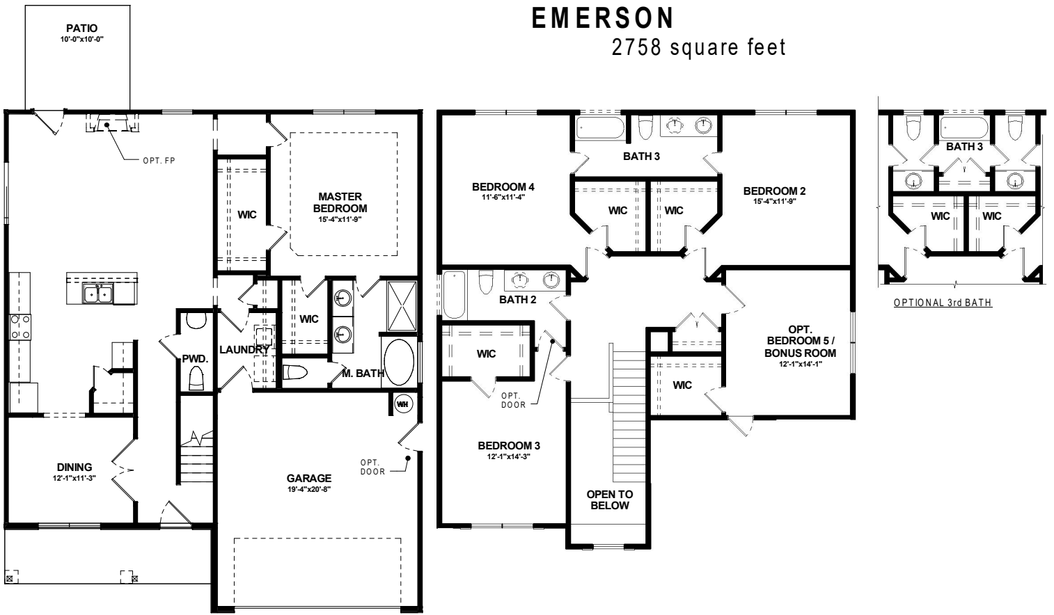
FIRST FLOOR
